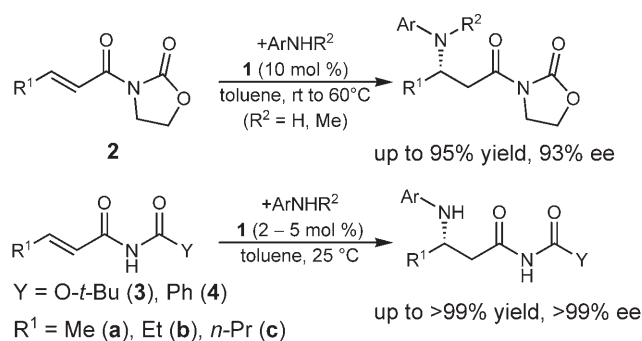
Scheme 1. Asymmetric aza-Michael reactions catalysed by palladium complex 1 .
