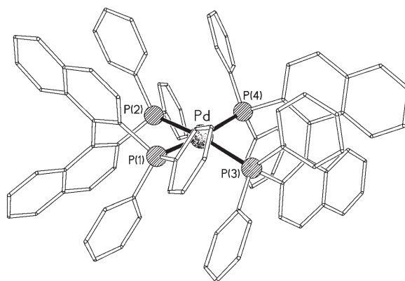
Figure 3. The molecular structure of the dication in 6 (the triflate counterions are not shown).
