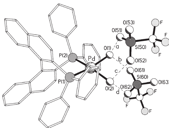
Figure 2. The molecular structure of 5 . The aqua...triflate hydrogen bonds have O...O separations (Å) of a ) 2.716(6), b ) 2.612(14), c ) 2.716(6) and d ) 2.994(10) Å.
