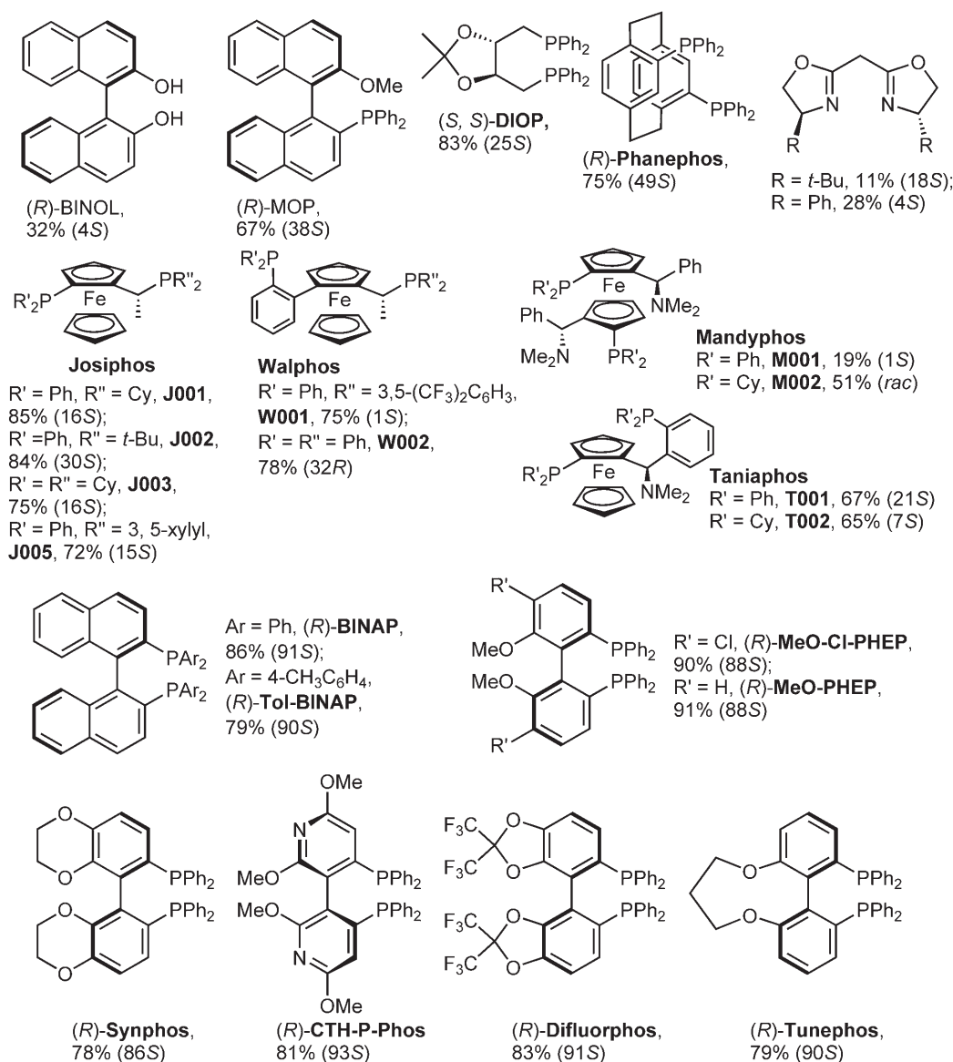
Figure 1. Evaluation of twenty-four commercially available ligands in the addition of aniline to 4a .
